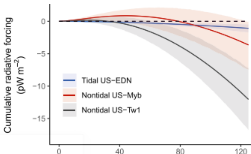
Figure 5. Modeled cross-over times for restored San Francisco Bay and Delta wetlands determined by the change in CH 4 and CO 2 dynamics of wetlands compared to previous land use (cumulative radiative forcing on the y-axis). X-axis represents time since restoration (years). Wetlands achieve a net cooling effect when the cumulative radiative forcing < 0. Factors such as salinity, previous land use, and accretion rates will influence crossover times. EDN = Eden Landing (Bay); Myb = Mayberry (Sherman Island, Delta); Tw1 = West Pond (Twitchell Island, Delta). Figure used with permission from Arias-Ortiz et al. (2021).
