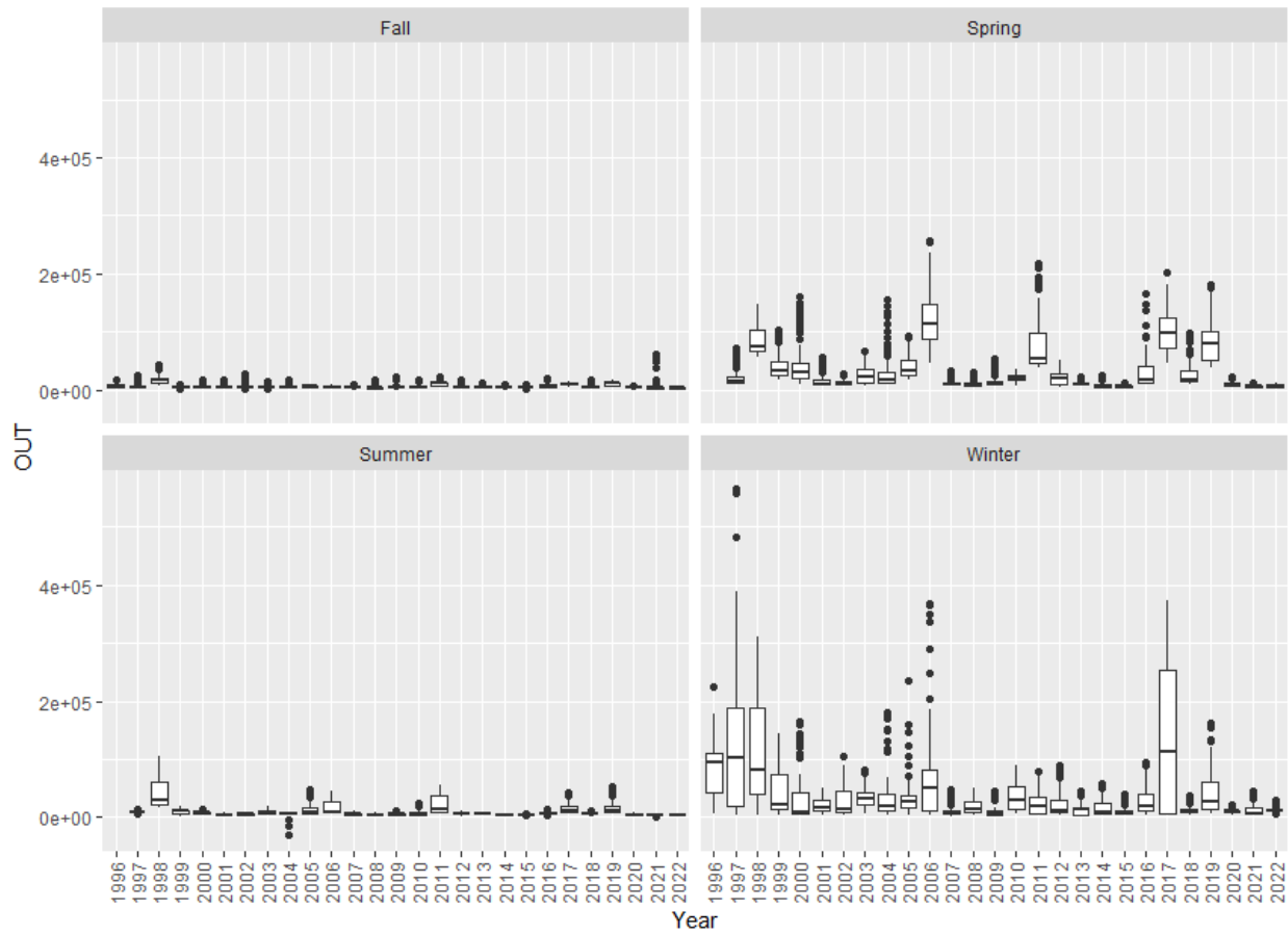
Figure 9-18. Boxplots for outflow at Chipps Island (from CDEC) from 1996-2022.
