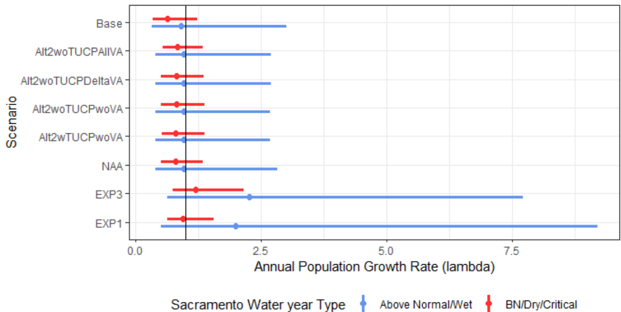
Figure 9-25. Geometric means (points) and full ranges (lines) of projected population growth rate ( \lambda ) by hydrology and covariate scenario (1995-2015; note that projection is initiated from the 2015 adult abundance index).
