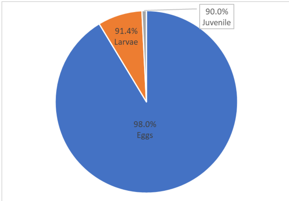
Figure 9-24. Delta Smelt Mortality by Life Stage Based on the U.S. Fish and Wildlife Service Adult Equivalents for Each Life Stage
