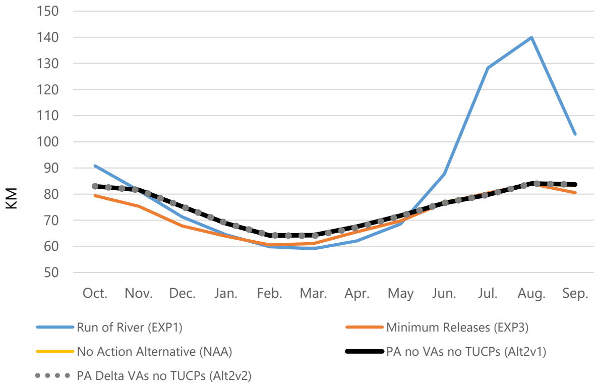
Figure 9-21. Average location of X2 under Run of the River, Minimum Releases, No Action, and the Proposed Action.
