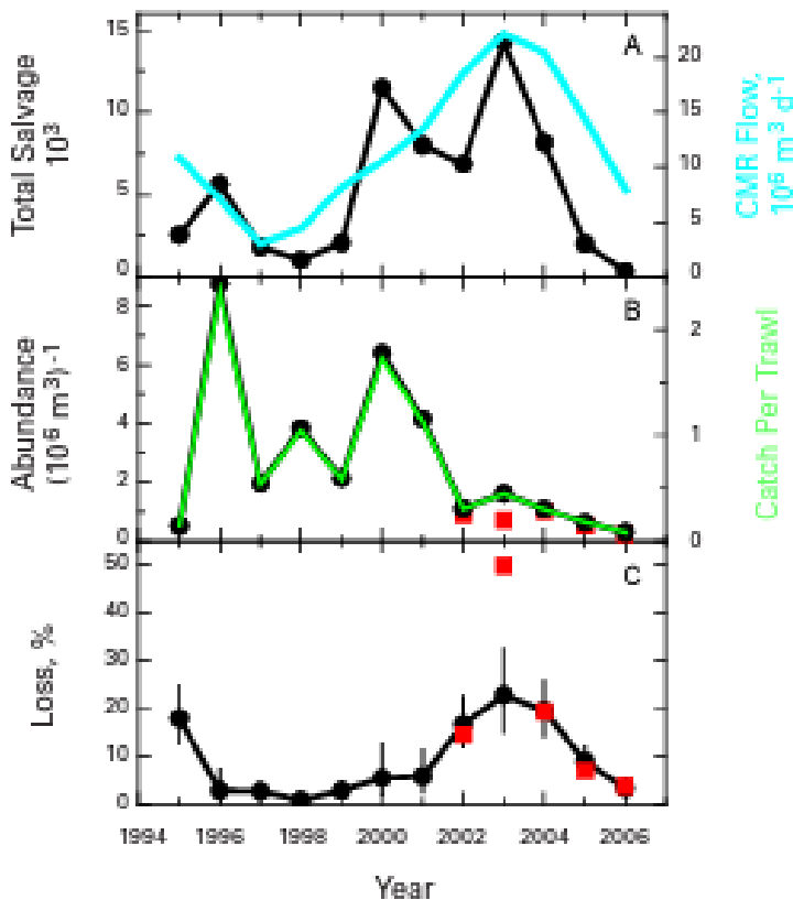
Figure 12. Reconstruction of export losses of adult delta smelt for 1995–2006. (A) Total salvage (line with circles) and Old and Middle River flow (line, right axis); (B) Predicted (line with circles) and measured (squares) population abundance, and mean catch per trawl for the fall trawl surveys in November and December (line, right axis); (C) Predicted (error bars, 5th and 95th percentiles) and measured (squares) proportional losses to export entrainment.
