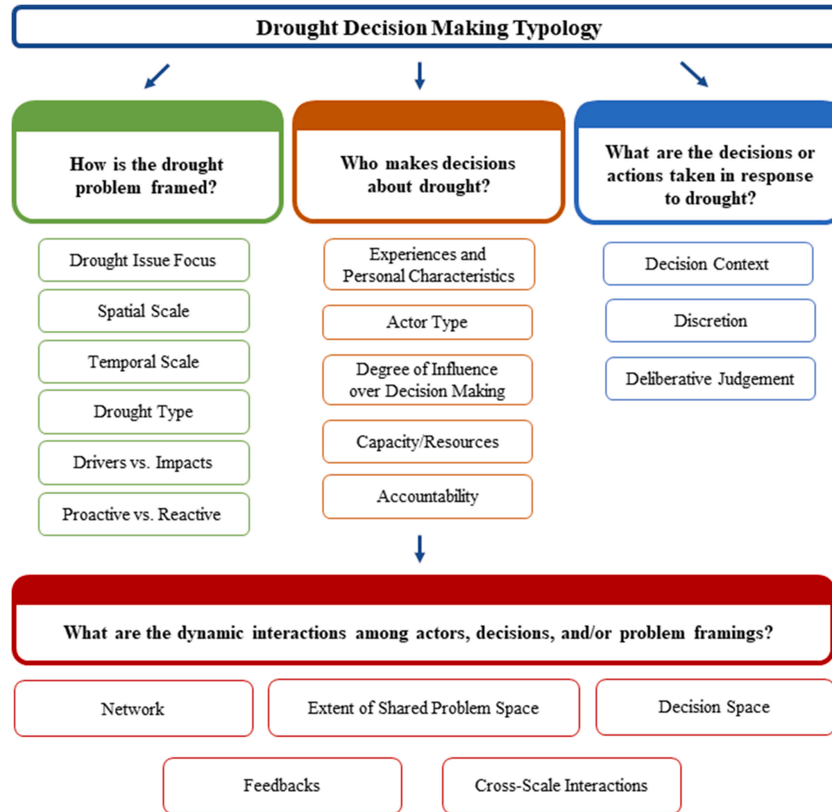
Figure 2 from Cravens, A. E., Henderson, J., Friedman, J., Burkardt, N., Cooper, A. E., Haigh, T., Hayes, M., McEvoy, J., Paladino, S., Wilke, A. K., & Wilmer, H. (2021, July 31). A typology of drought decision making: Synthesizing across cases to understand drought preparedness and response actions . Weather and Climate Extremes . Retrieved October 5, 2021, from https://www.sciencedirect.com/science/article/pii/S2212094721000542 .
